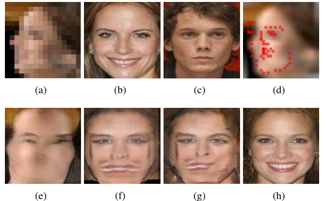
Fig. 1. Comparison with the combination of face hallucination [2] and frontalization [1] methods. (a) 16 \times 16 LR non-frontal input image. (b) 128 \times 128 HR original frontal image (not available in training). (c) The best possible match to the given LR image in the dataset after compensating for in-plane rotations by STN_0 [3]. (d) Detected landmarks by [4] after bicubic upsampling. (e) Result obtained by applying [1] first and then [2]. In [2], the first decoder and encoder are used to reduce image noise. Hereby, we only use the second decoder of [2] for super-resolving LR faces. (f) Result obtained by applying [2] first and then [1]. (g) Image generated by [2], which is retrained with LR non-frontal and HR frontal face images. (h) Our result.
