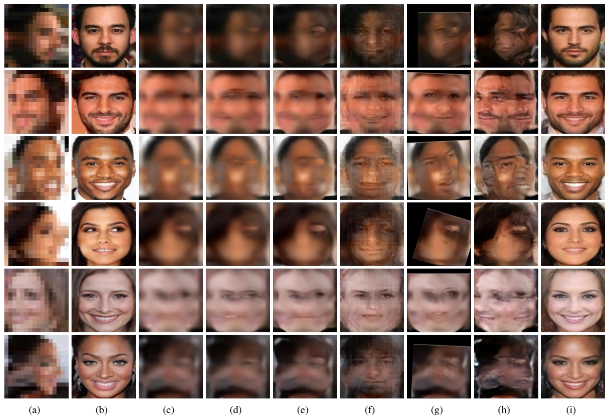
Fig. 8. Results of the state-of-the-art methods for frontalization followed by hallucination . Columns: (a) Unaligned non-frontal LR inputs. (b) Original frontal HR images. (c) [1] + bicubic interpolation. (d) [1] + [59]. (e) [1] + [60]. (f) [1] + [17]. (g) [1] + [51]. (h) [1] + [2]. (i) Our method.
